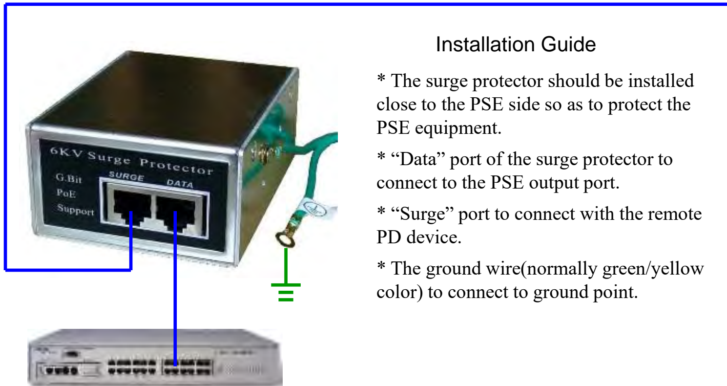
PSE: PoE Switch or PoE Midspan
